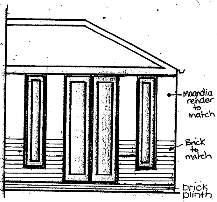
South elevation
