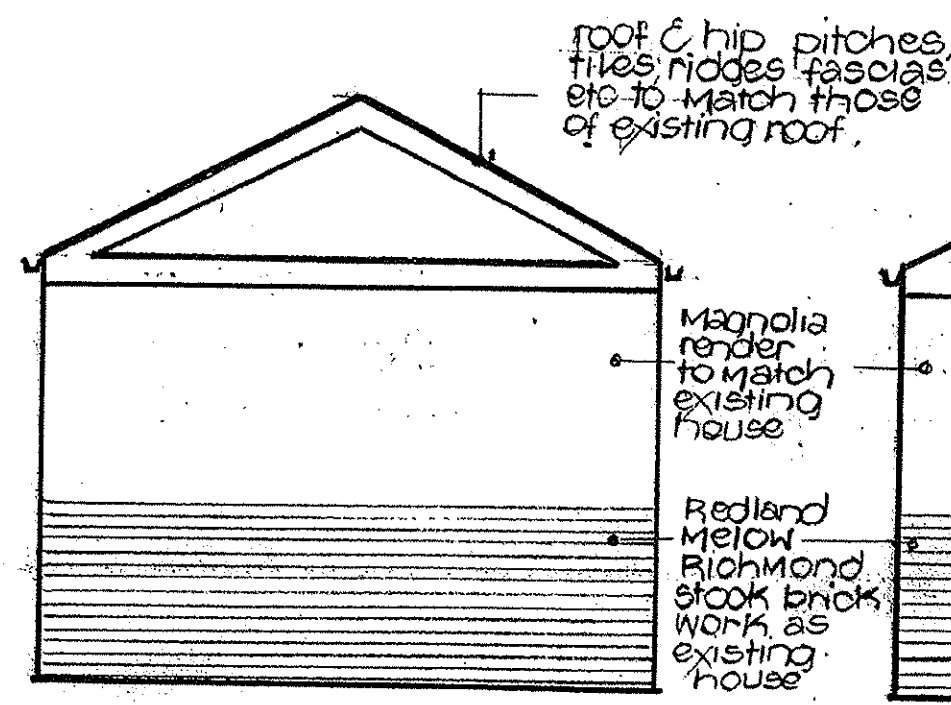
east elevation/gable
